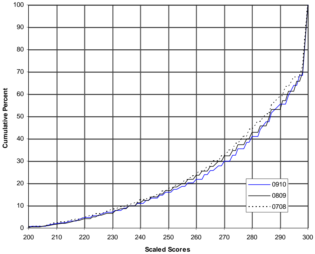
REA07 Scaled Scores
